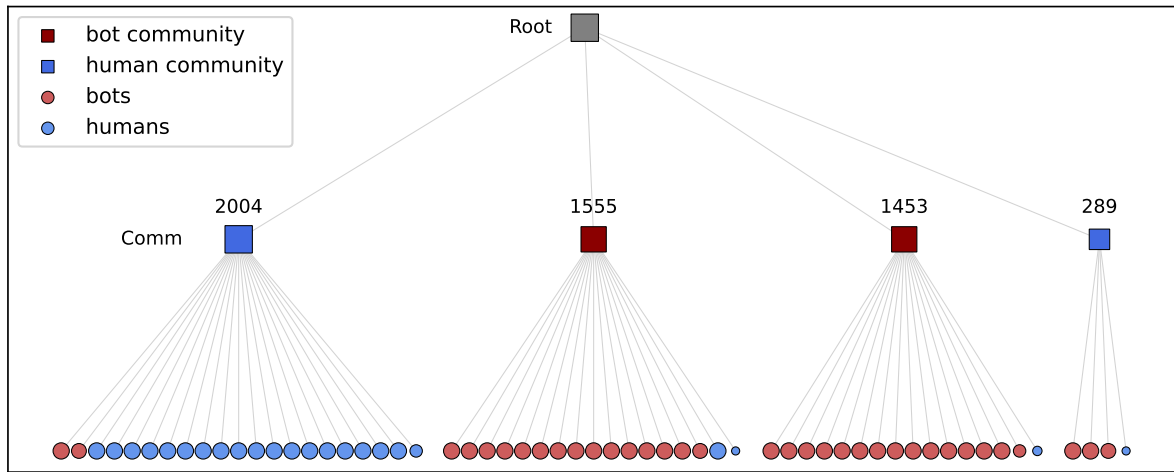
(c) The optimal encoding tree of Cresci-2015 dataset in UnDBot (square tree nodes are communities, circular leaf nodes are social users, and the size of the nodes indicates the number of social users. For visualization, each large leaf node represents 100 social users of Cresci-2015).
