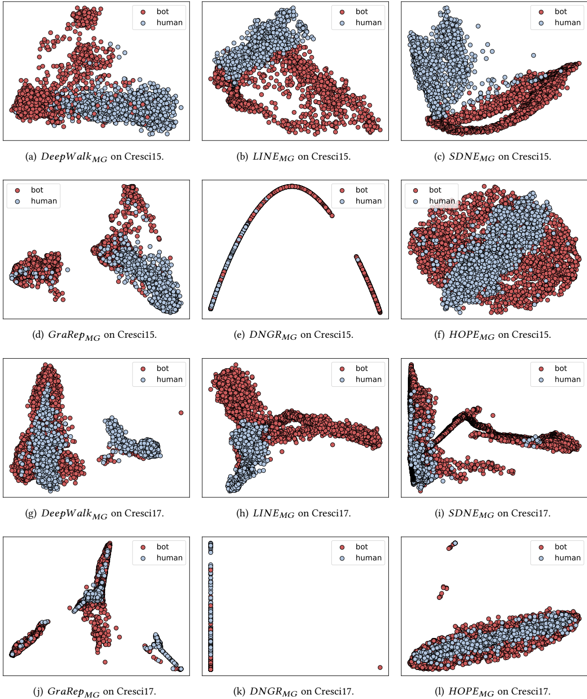
Fig. 4. Distribution of user embeddings generated by unsupervised graph learning models on the Cresci-2015 and Cresci-2017 datasets.
